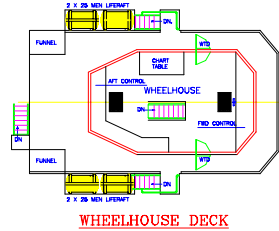
WHEELHOUSE DECK
