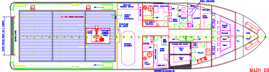
MAIN DECK
