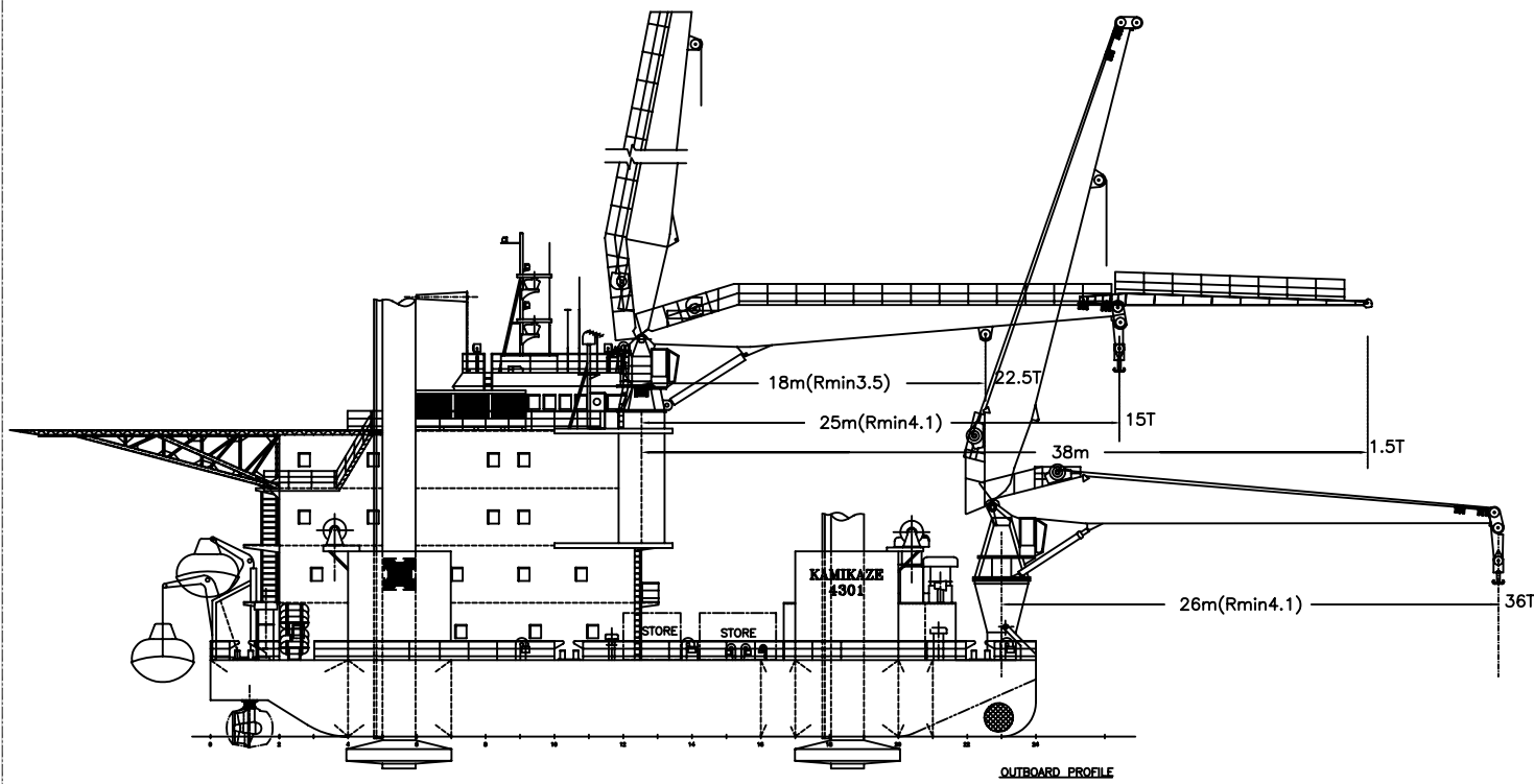
OUTBOARD PROFILE
